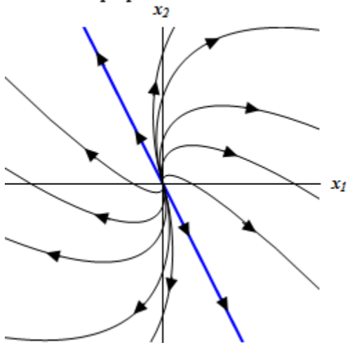
Improper Node - Unstable
