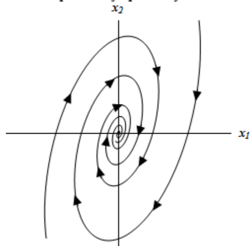
Spiral - Asymptotically Stable
