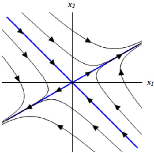
Saddle Point - Unstable
