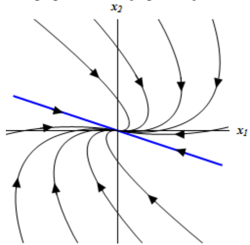
Improper Node - Asymptotically Stable
